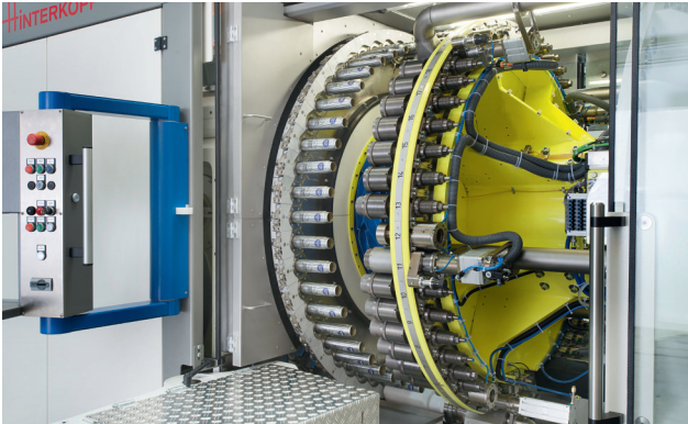
The necking machine N50.3 from Hinterkopf with its 50 working stations opens up entirely new possibilities for shaping.
